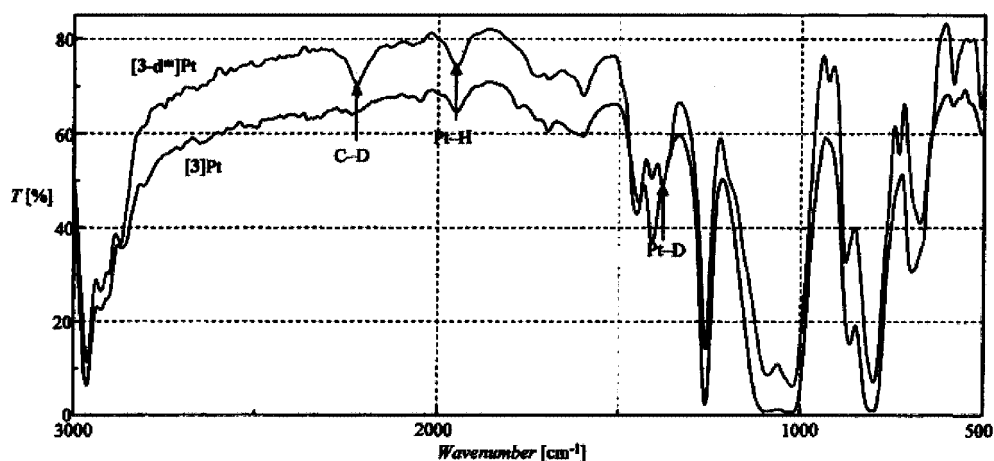
Figure 9. FT-IR spectra for [D m -3]Pt and [3]Pt.
