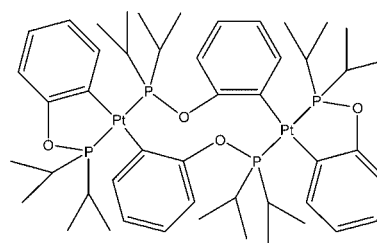
Figure 13. Proposed structure of the second product found in the course of cis/trans isomerization of cis -[1*]Pt based on the ^{31}\text{P} NMR results.
