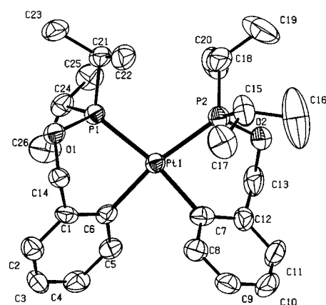
Figure 12. ORTEP style plot of the compound cis -[3*]Pt in the solid. Thermal ellipsoids are drawn at the 50% probability level. Hydrogen atoms have been omitted for clarity.
