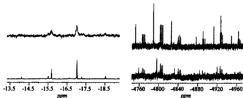
Figure 6. Excerpt of the ^1\text{H} (bottom left), ^2\text{H} (top left), ^{195}\text{Pt} (top right), and ^{195}\text{Pt}\{^1\text{H}\} (bottom right) NMR spectra showing the Pt–H(D) signals.
