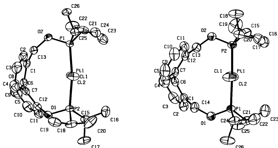
Figure 3. ORTEP style plot of the compounds trans -[2]PtCl 2 (left) and trans -[3]PtCl 2 (right) in the solid. Thermal ellipsoids are drawn at the 50% probability level. Hydrogen atoms have been omitted for clarity.
