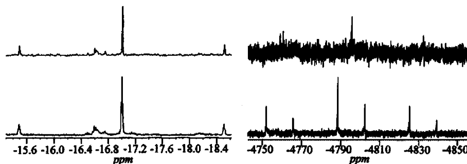
Figure 5. Portions of the ^1\text{H} (left) and ^{195}\text{Pt} (right) NMR spectra showing the Pt–H signals. Top: ^1\text{H}\{^{31}\text{P}\} and ^{195}\text{Pt}\{^1\text{H}\} .
