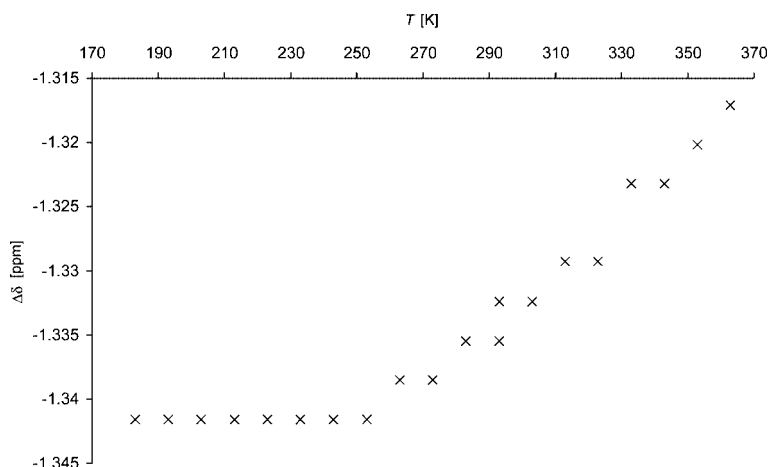
Figure 7. Temperature dependence of the chemical-shift difference, \Delta\delta , in the ^1\text{H} NMR spectrum between the two peaks at about \delta = -15.5 and -17 ppm.
