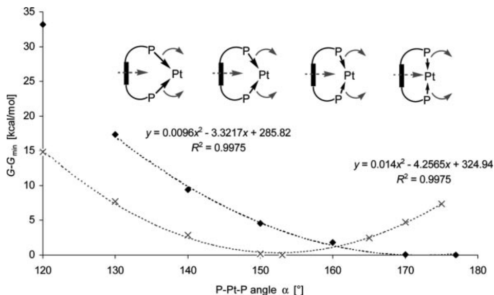
Figure 1. Potential of the P–Pt–P bending vibration for [1]Pt (×) and [3]Pt (♦) calculated using DFT theory (functional: B3PW91; basis set: LANL2DZ).
