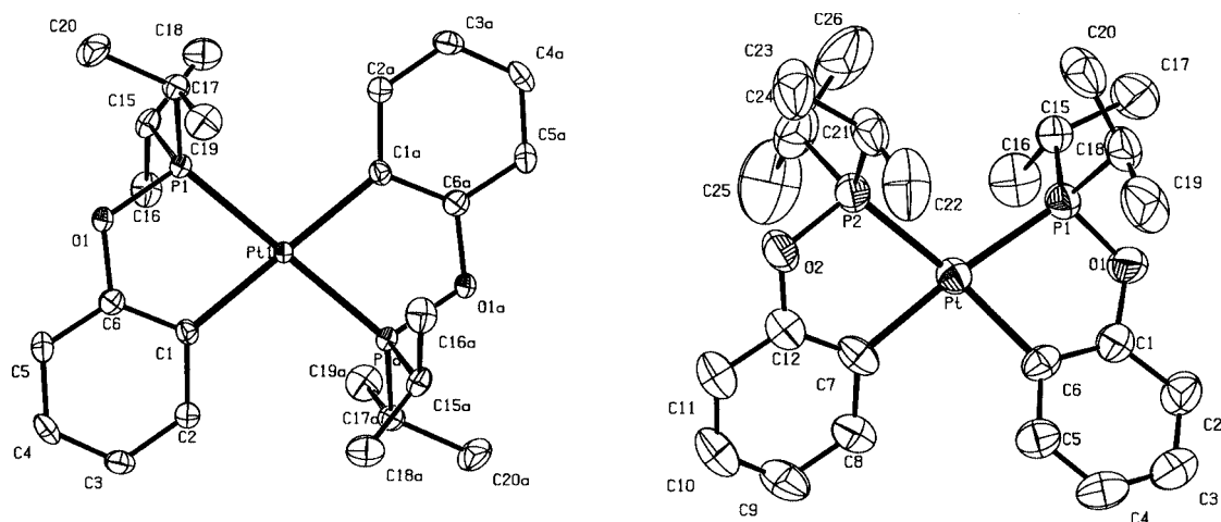
Figure 14. ORTEP style plot of the compounds trans -[1*]Pt (left) and cis -[1*]Pt (right) in the solid. Thermal ellipsoids are drawn at the 50% probability level. Hydrogen atoms have been omitted for clarity.
