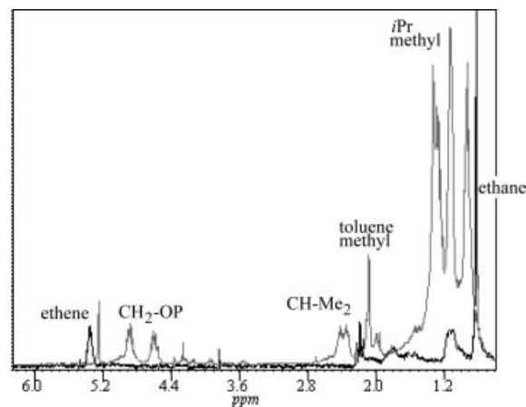
Figure 8. ^1\text{H} NMR spectrum (grey) of [3]\text{Pt} in [\text{D}_8]\text{toluene} and the ^2\text{H} NMR spectrum of [\text{D}_m\text{-}3]\text{Pt} ( m : number of incorporated deuterium atoms into the ligand in the course of the thermolysis) in non-deuterated toluene (black) in the region between 0.7 and 6 ppm.
