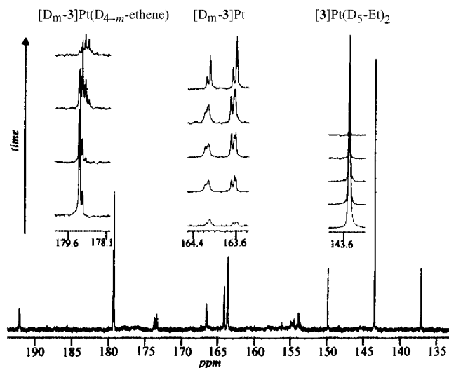
Figure 10. Time-dependent 31 P NMR spectra for the thermolysis of [3]Pt(D 5 -Et) 2 showing the scrambling of deuterium into the ligand during the reaction.
