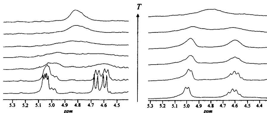
Figure 11. Results of the variable-temperature ^1\text{H} NMR measurements for the \text{OCH}_2 protons in cis -[3*]Pt (left) and trans -[3*]Pt (right) between -90 and 100^\circ\text{C} .
