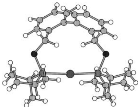
Figure 2. Plot of the calculated minimum structure of [3]Pt.
